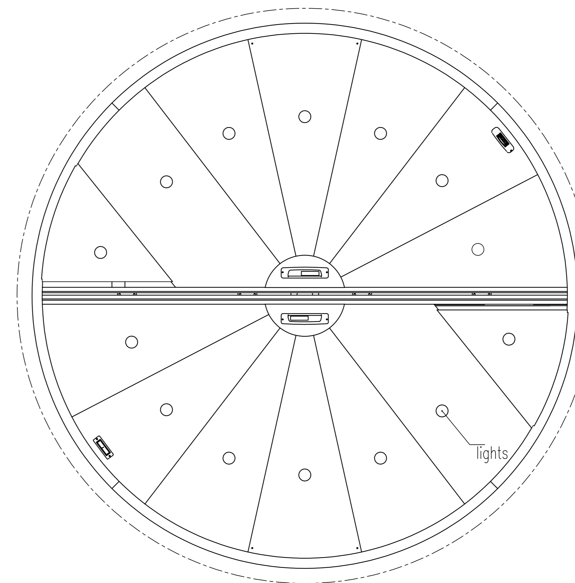
Top view of ceiling
